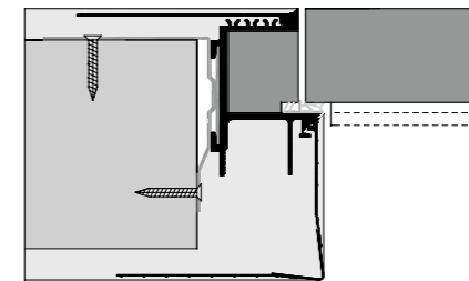
Invisible TUT45 frame, Out-swing, Door thickness: 45mm
