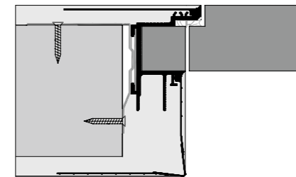
Invisible TUS50 frame, In-swing, Door thickness: 50mm
