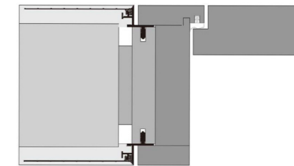
TL profile with wooden frame
