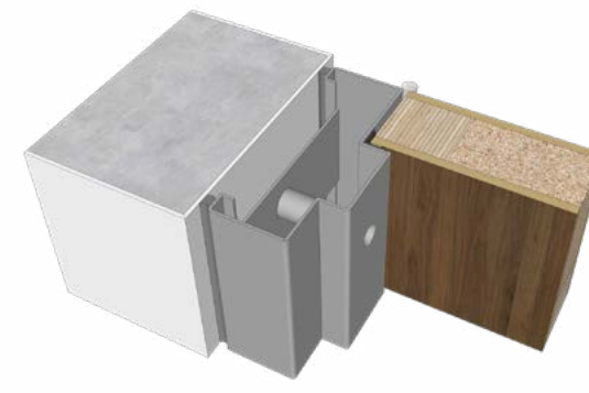
CMU wall Hollow metal frame with dimpled anchor
