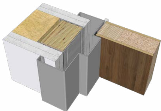
Drywall Hollow metal frame KD or welded
